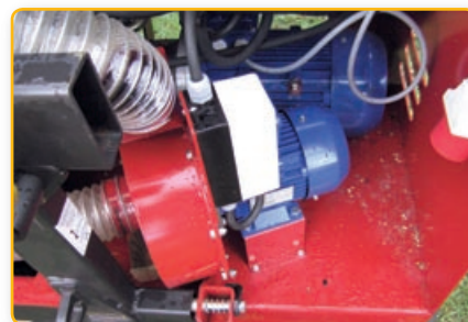
Sawdust extractor: The machine can also be delivered with electric or hydraulic sawdust suction.
